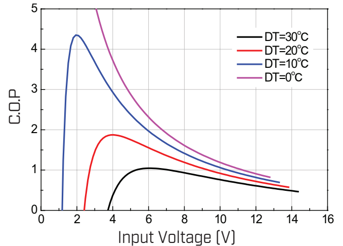
COP Vs. Input Voltage, V ( \Delta T=0\sim 30^\circ C )
