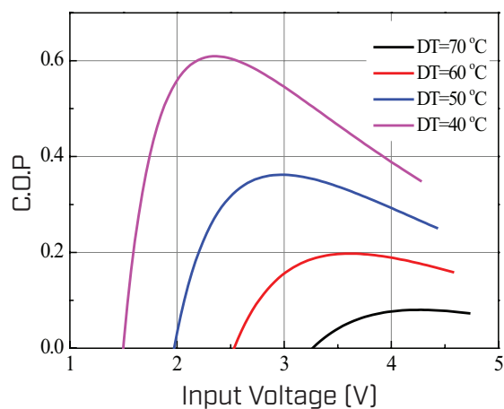
COP Vs. Input Voltage, V ( \Delta T=40\sim70^\circ\text{C} )
